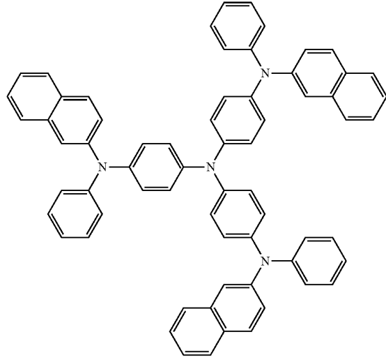
2T-NATA
