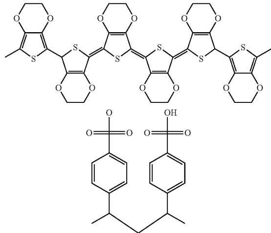
PEDOT/PSS
